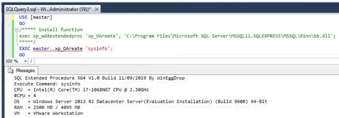
Reproduced SQLMaggie backdoor command
