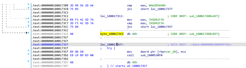
Figure 34. Antidebugging method
