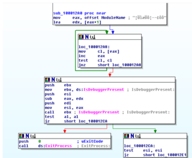
Figure 19. The anti-debugging feature in payload32.dll.
