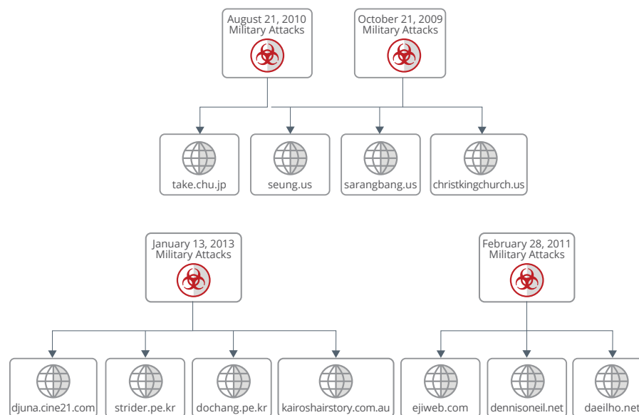
Figure 23. Encrypted data exfiltration network.
