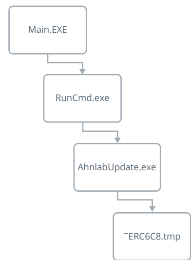
Figure 21. TDrop disguises its presence by appearing to be a security product.
