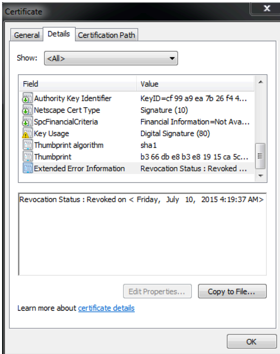
Figure 6. Certificate revocation
