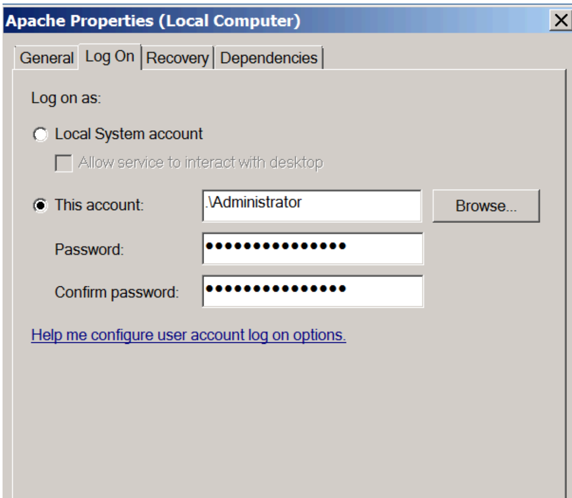
Apache Service Running as Administrator
