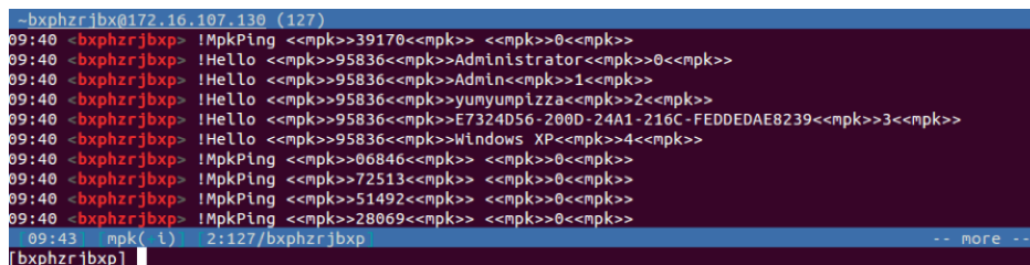
Figure 7 Initial private messages sent from MPK to the IRC C2 server
