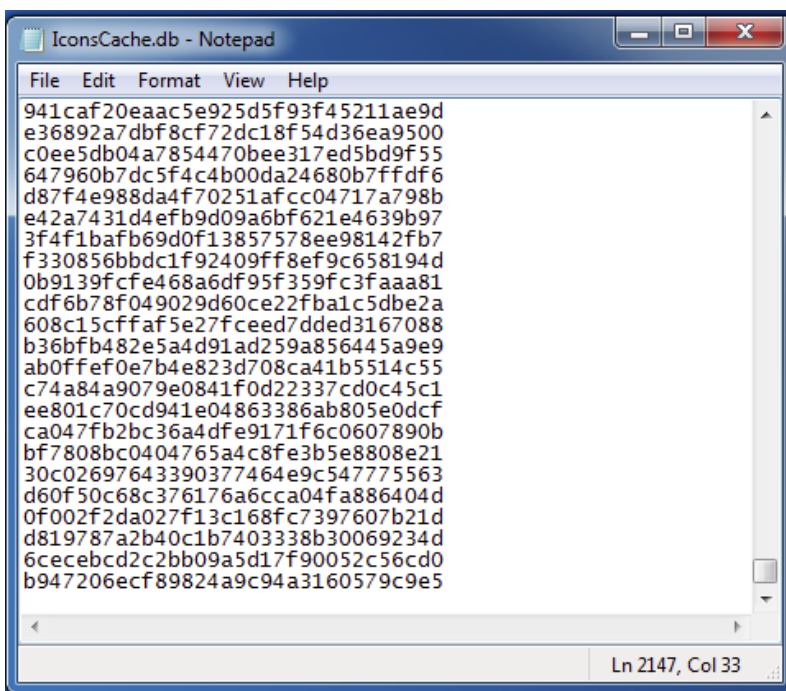
Figure 9. IconsCache.db contents.
