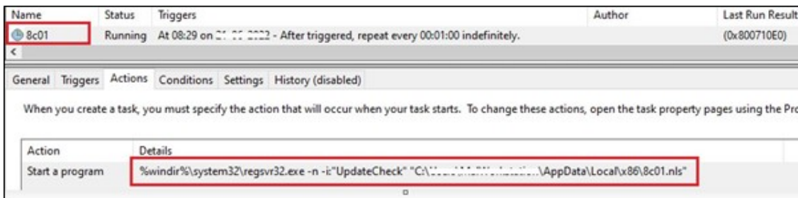
Figure 10 – Scheduled Task Entry for Persistence
