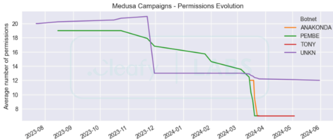
Figure 7 - Evolution of permission over time
