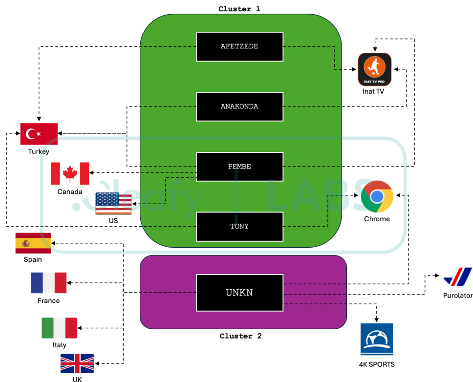
Figure 6 - Characteristics of the five botnets
