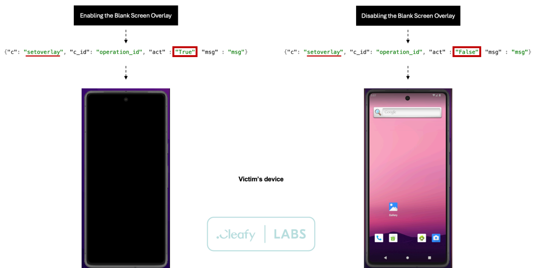
Figure 9 - Command “setoverlay” in action
