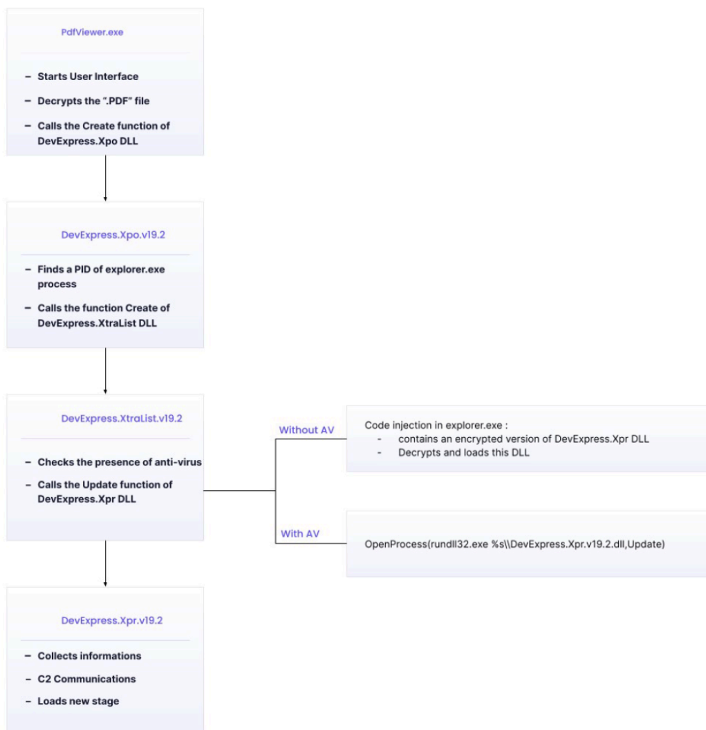
Figure 4. Windows RustBucket execution flow chart
