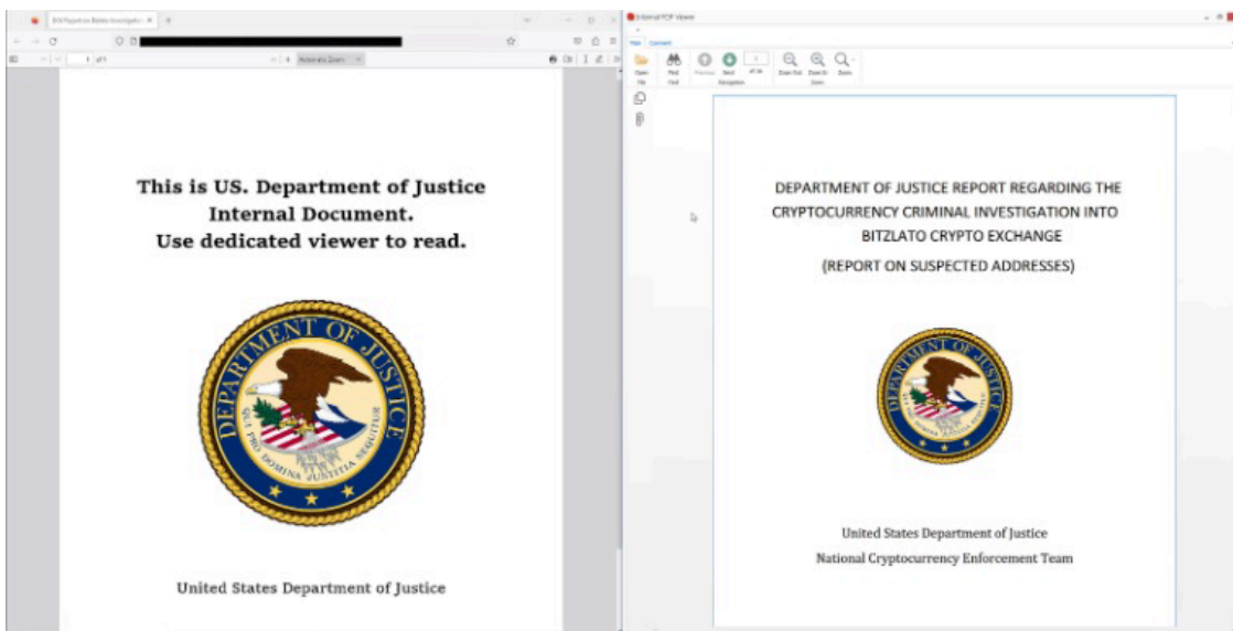
Figure 3. (left) Key PDF document opened in Firefox, (right) Key PDF document opened in the Internal PDF viewer
