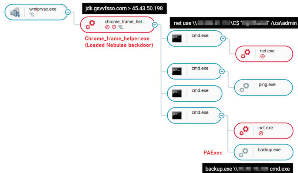
Nebulae Backdoor execution as seen in the Cybereason Defense Platform
