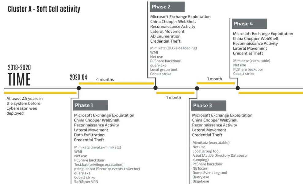
Timeline of the attack - Cluster 1
