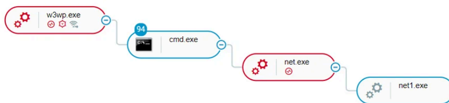
China Chopper WebShell activity as seen in the Cybereason Defense Platform
