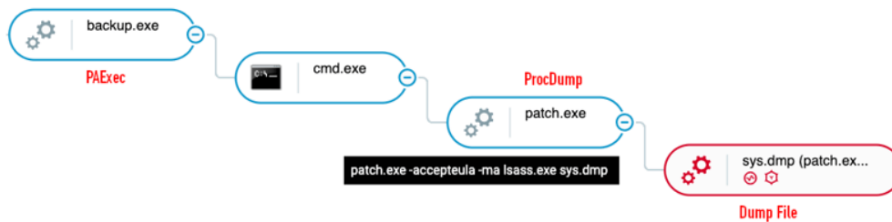
PAExec and ProcDump execution as seen in the Cybereason Defense Platform
