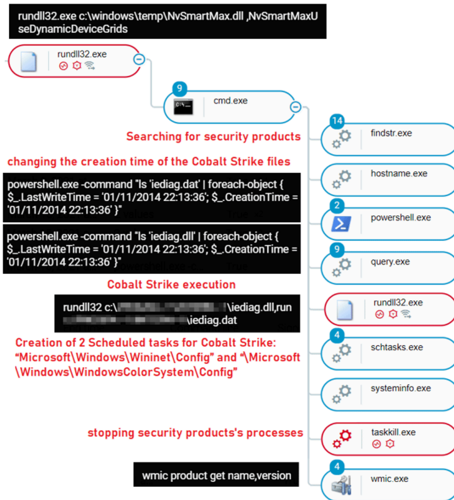
The execution of the PcShare backdoor as seen in the Cybereason Defense Platform
