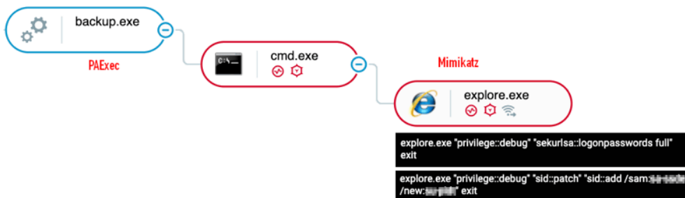
PAExec and Mimikatz execution as seen in the Cybereason Defense Platform
