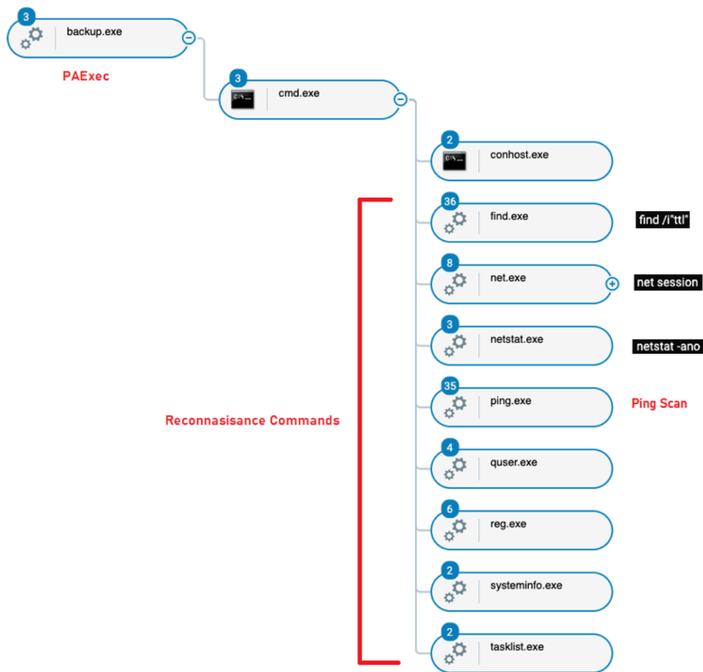
Execution of legitimate tools for reconnaissance and lateral movement as seen in the Cybereason Defense Platform
