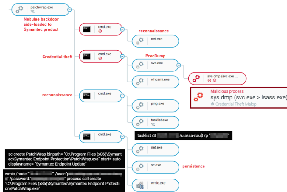
Nebulae Backdoor execution of various tasks as seen in the Cybereason Defense Platform
