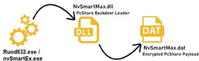
PcShare execution graph
