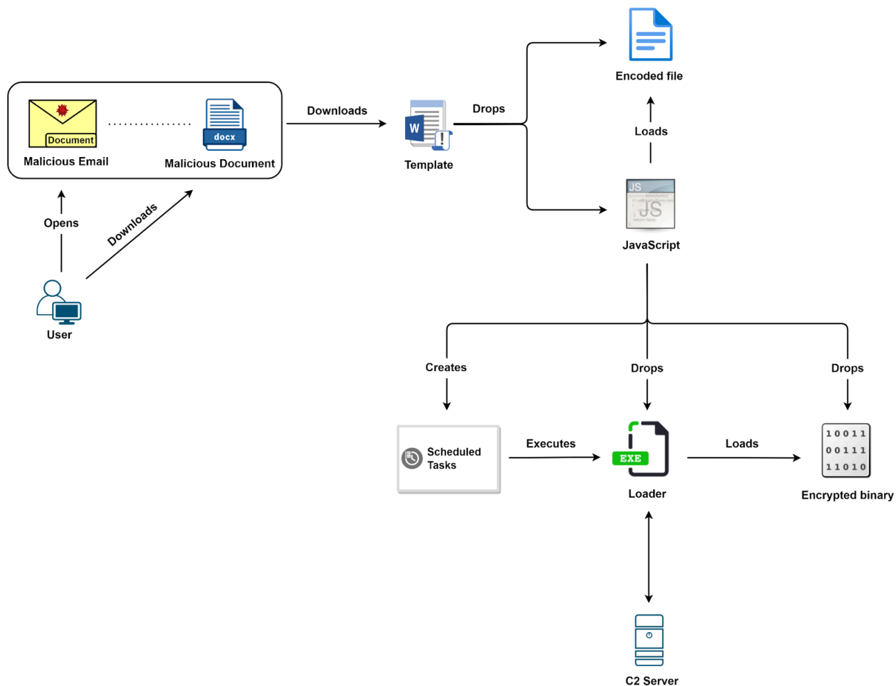
Figure 1: Attack chain
