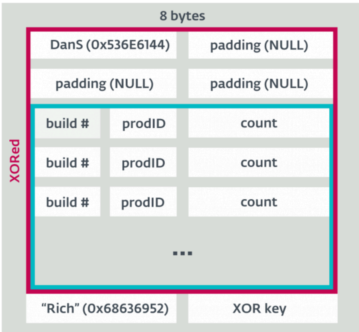
4: The unencrypted Rich Headers structure.
