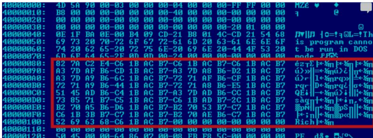
Figure 1: PE binary with Rich Headers highlighted.
