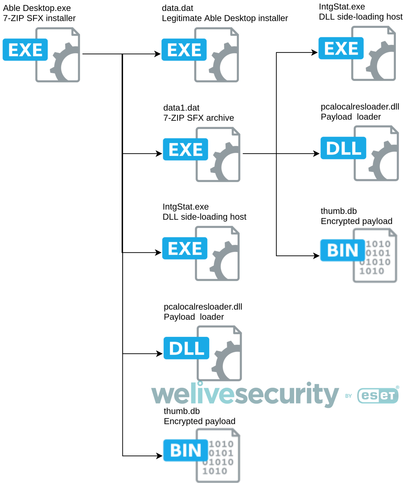
Figure 5. Trojanized Able Desktop installer content
