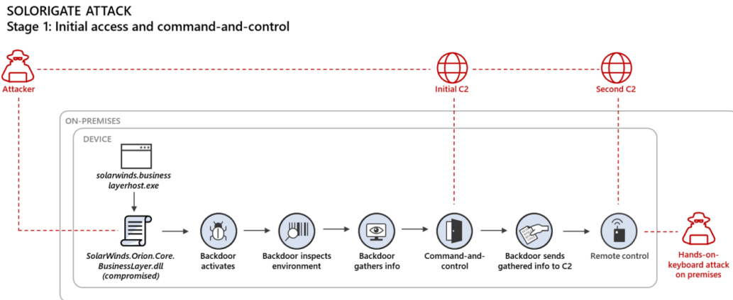
Figure 7. Solorigate attack chain: Initial access and command-and-control
