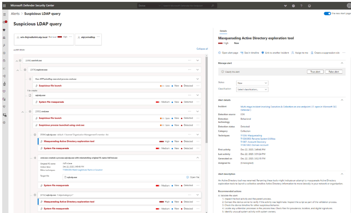
Figure 11. Microsoft Defender for Endpoint detects usage of masquerading exploration tools
