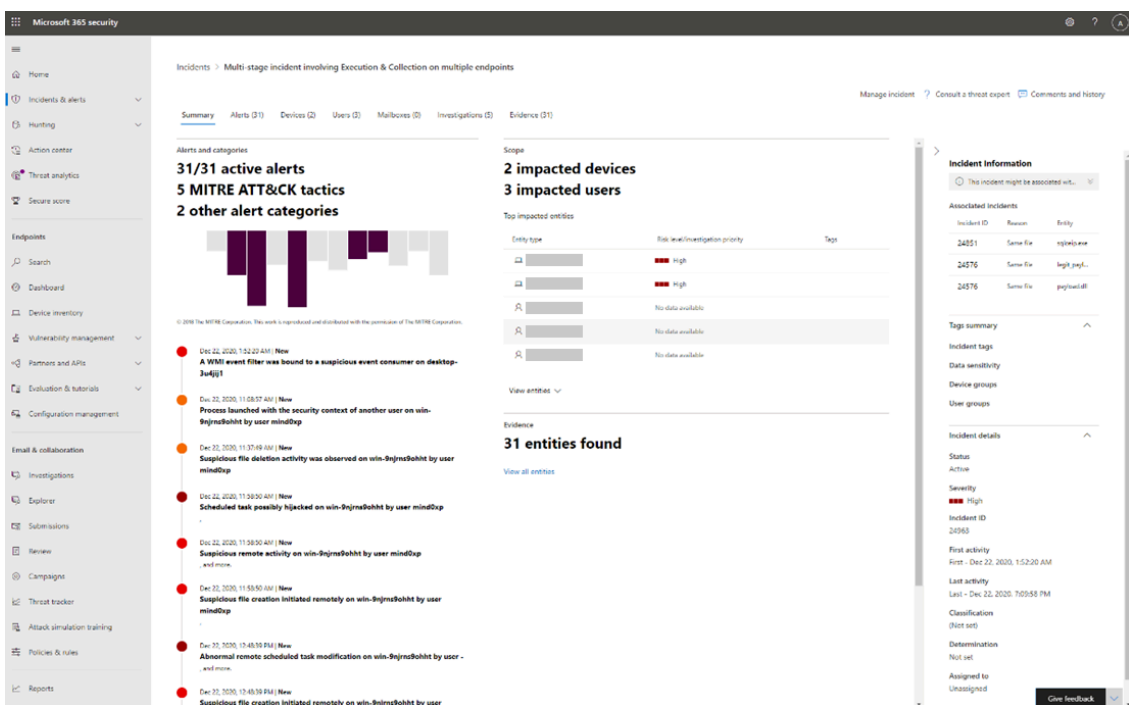
Figure 5. Consolidated Incident view for Solorigate
