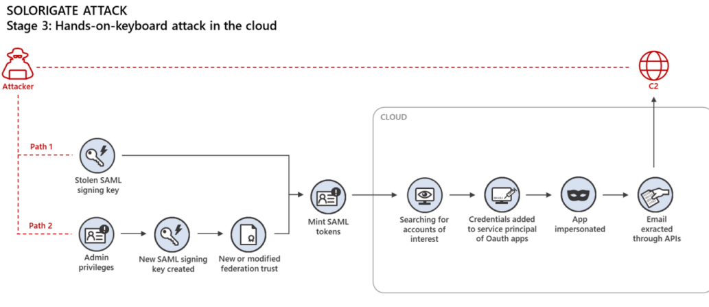
Figure 17. Solorigate attack chain: Hands-on-keyboard attack in the cloud
