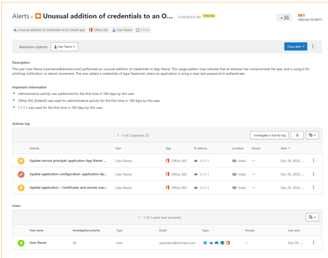
Figure 18. Microsoft Defender Cloud App Security alert for unusual addition of credentials to an OAuth app
