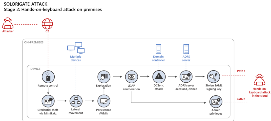
Figure 10. Solorigate attack chain: Hands-on-keyboard attack on premises
