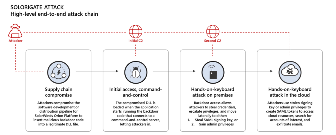
Figure 1. High-level end-to-end Solorigate attack chain
