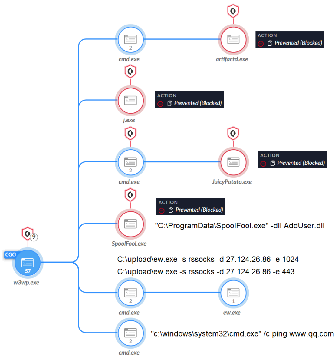
Figure 2. Process tree of Cobalt Strike, the Potato Suite, SpoolFool and EarthWorm.
