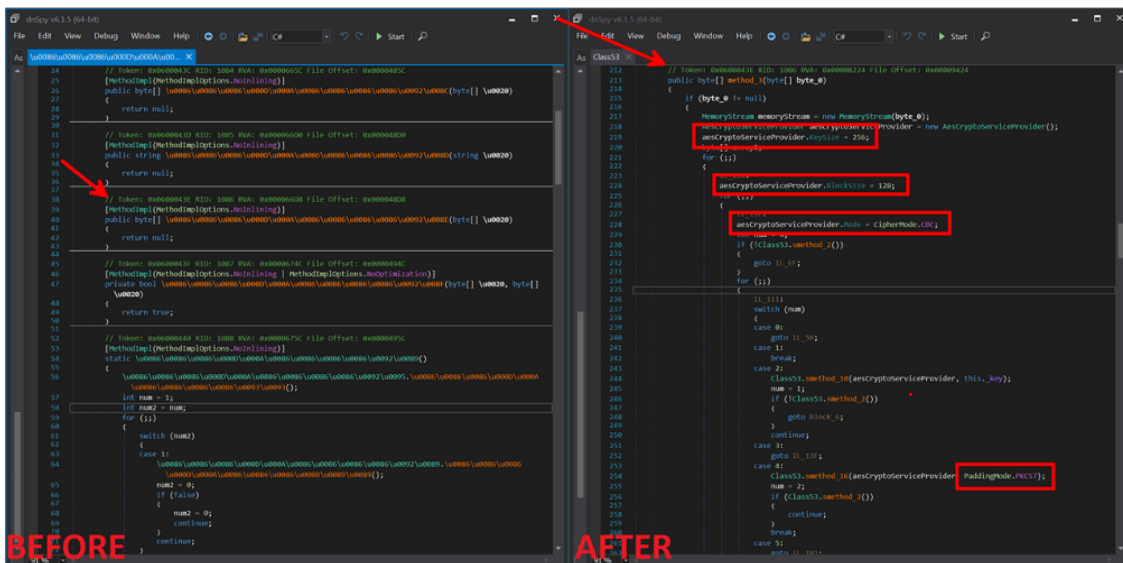
Figure 17: Method 0x0600043 before and after fixing the assembly
