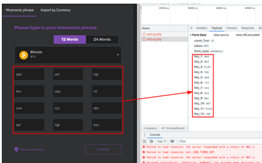
Figure 16. A mnemonic phrase being sent to the server controlled by the malicious actors behind Cryptomining Farm Your own Coin
