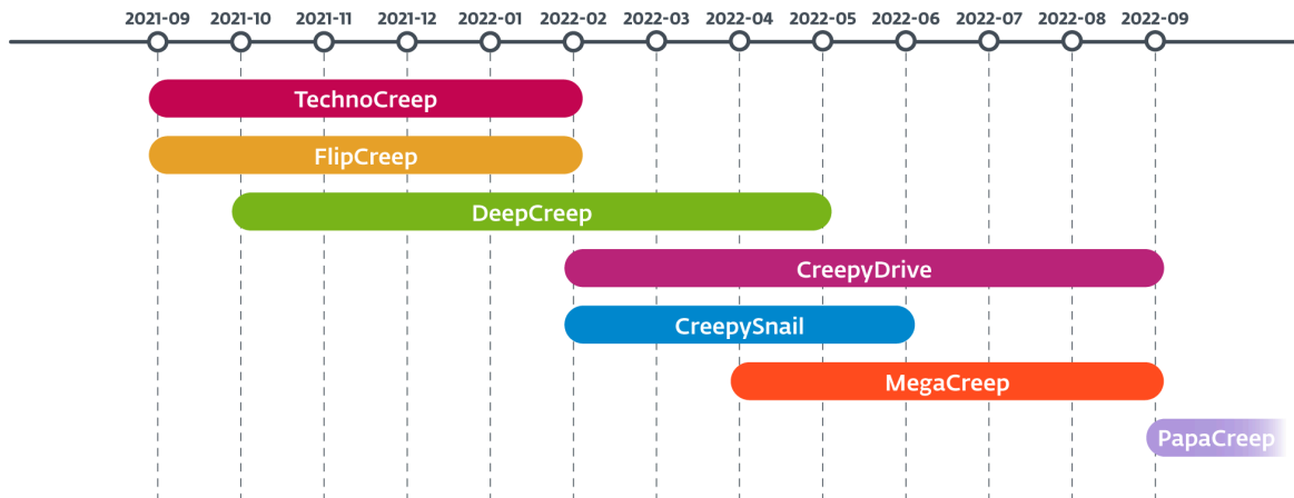
Figure 1. Timeline of observed backdoors deployed by POLONIUM
