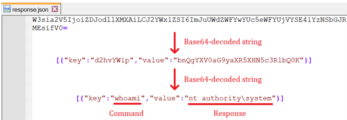
Figure 3. Execution log of a command and its output
