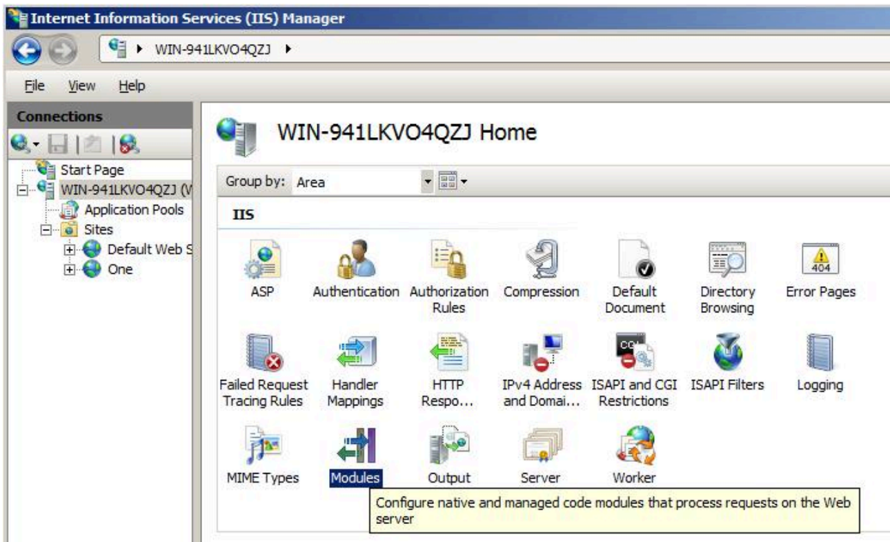
Figure 1: IIS Manager
