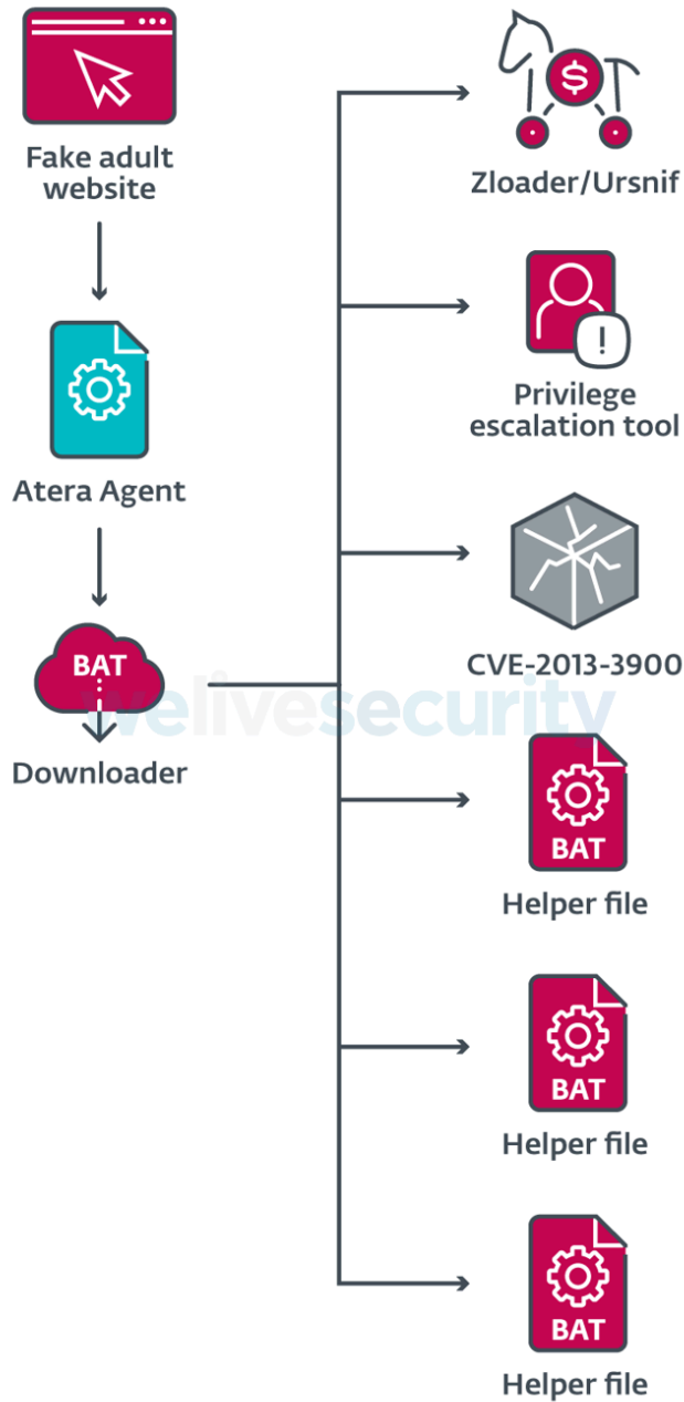
Figure 8. Typical distribution method using Atera Agent
