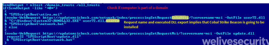
Figure 5. PowerShell script responsible for Cobalt Strike Beacon installation
