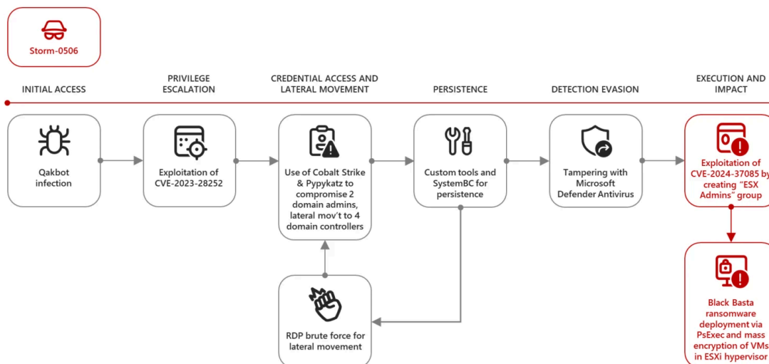
Figure 2. Storm-0506 attack chain
