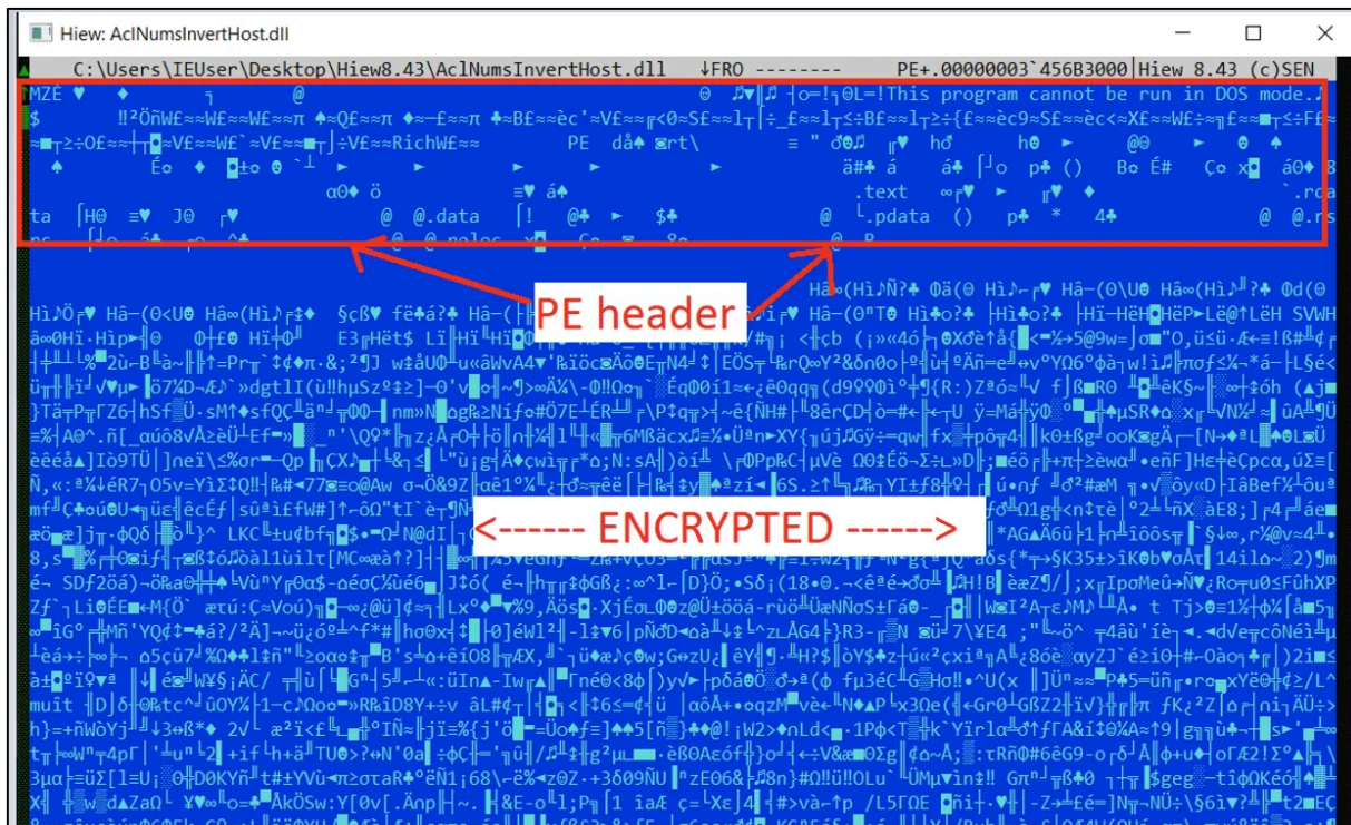
Figure 10: Encrypted code section of the AclNumsInvertHost.dll executed as part of the main threat actor's scheduled task persistence.
