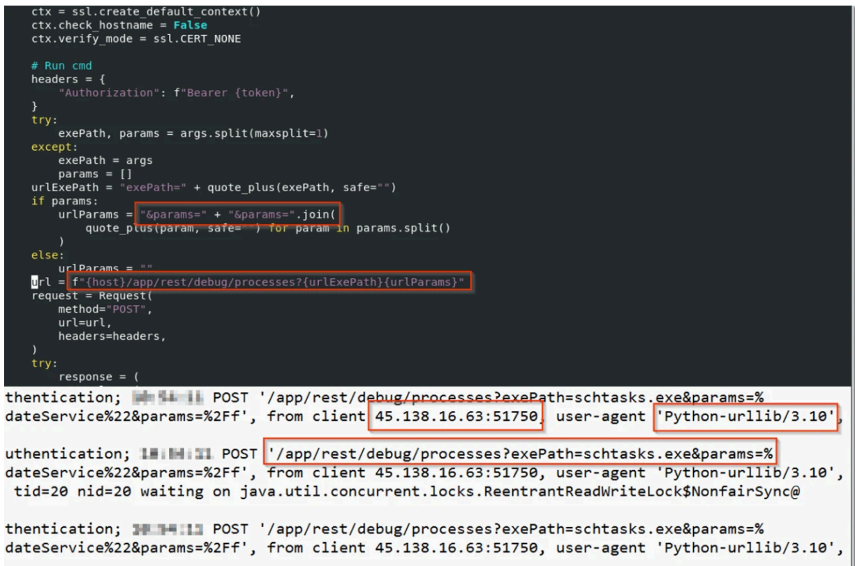
Figure 8: A snippet of code from poc.py found on the C2 web server, and a snippet of the TeamCity log showing a similar request received by the victim during exploitation.
