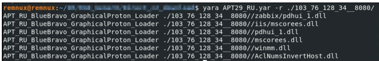
Figure 11: Yara rule for GraphicalProton matched against multiple DLL files found on the main threat actor opendir server.
