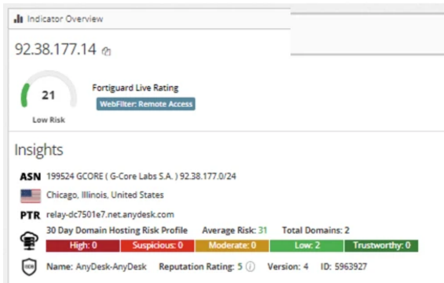
Figure 24: FortiGuard CTS screen with information about AnyDesk relay IP address.
