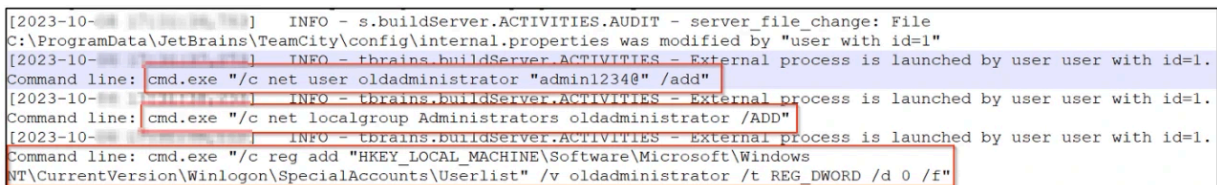
Figure 15: Extract from the TeamCity application logs showing the commands used to create a new local Windows user on the victim endpoint.
