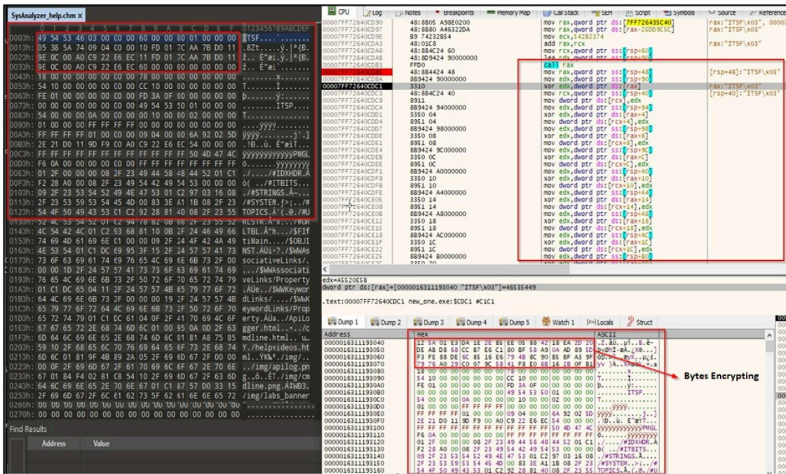
Figure 10 – Encryption Routine
