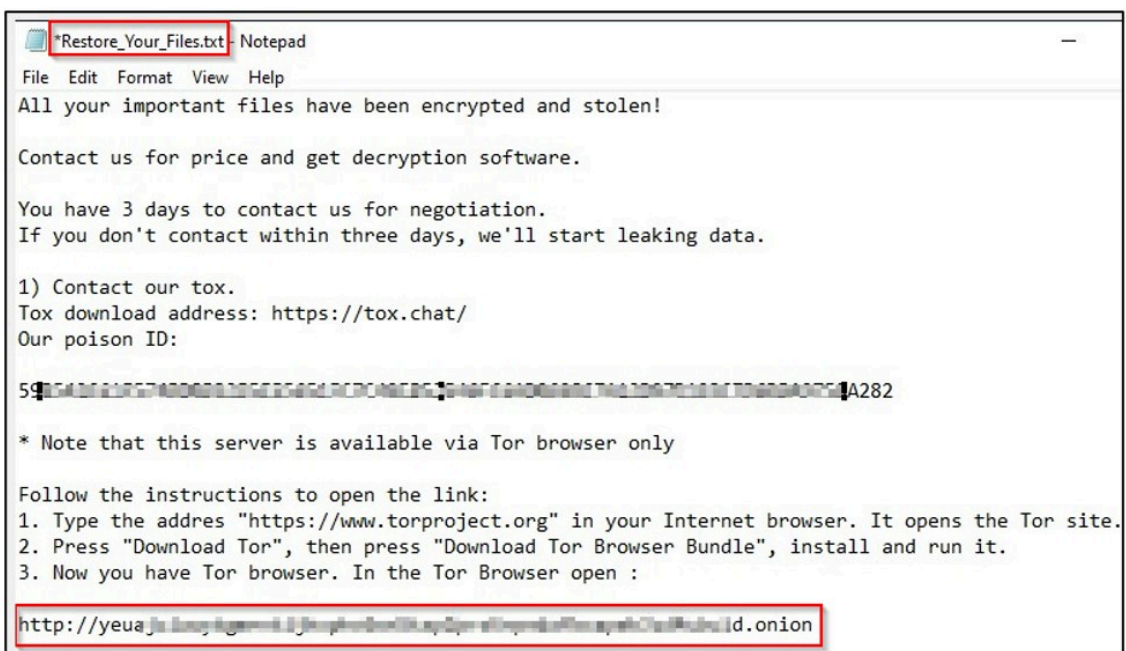
Figure 14 – Ransom Note
