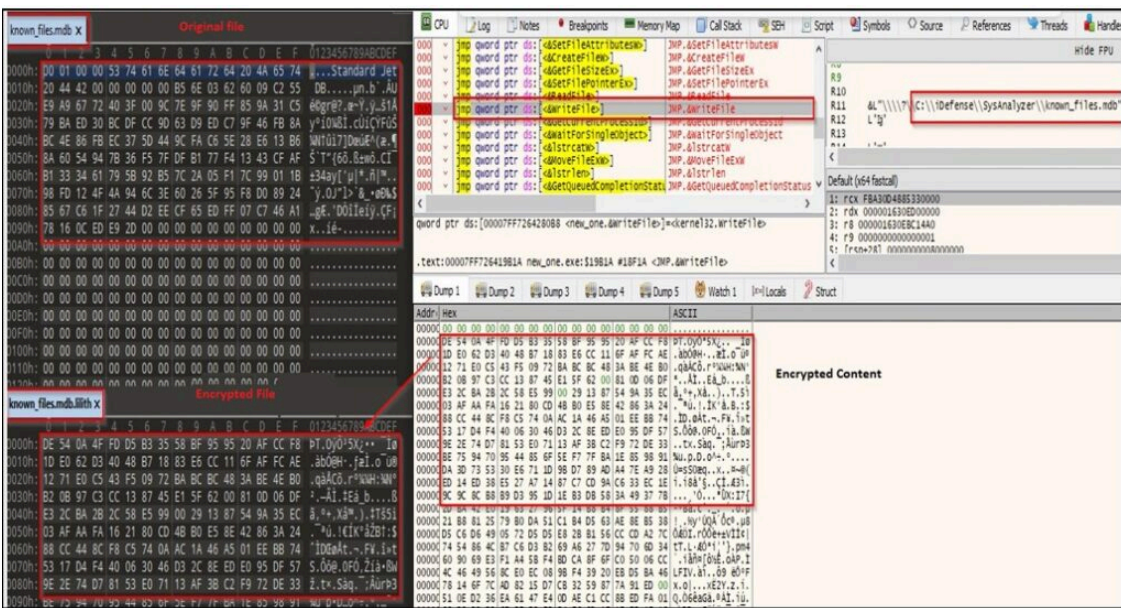
Figure 11 – WriteFile() Operation
