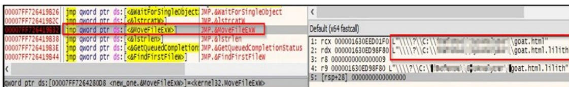
Figure 12 – MoveFileExW() API
