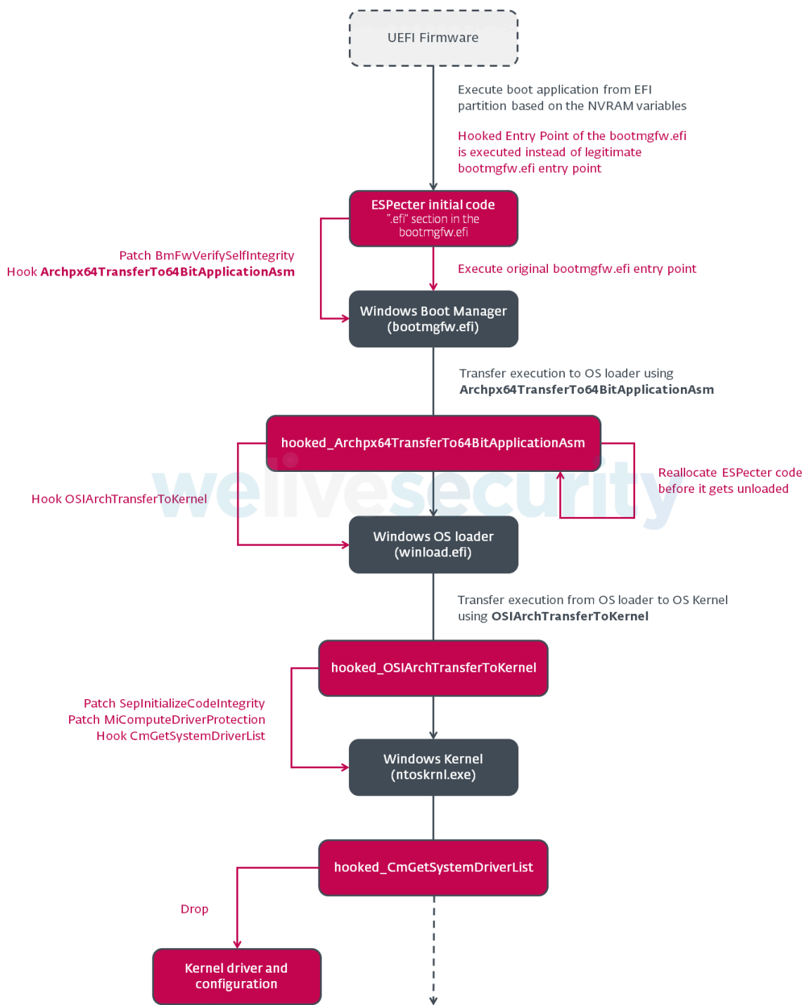
Figure 5. Boot flow modified by ESpecter
