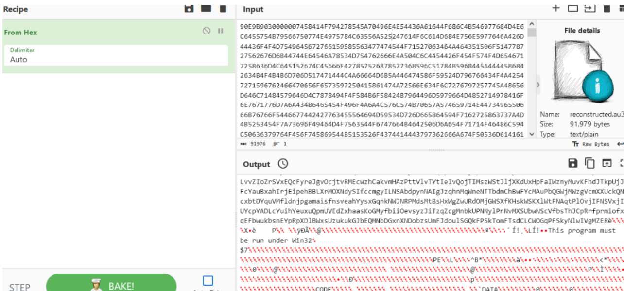
Figure 29: Decoding the Included Shellcode
