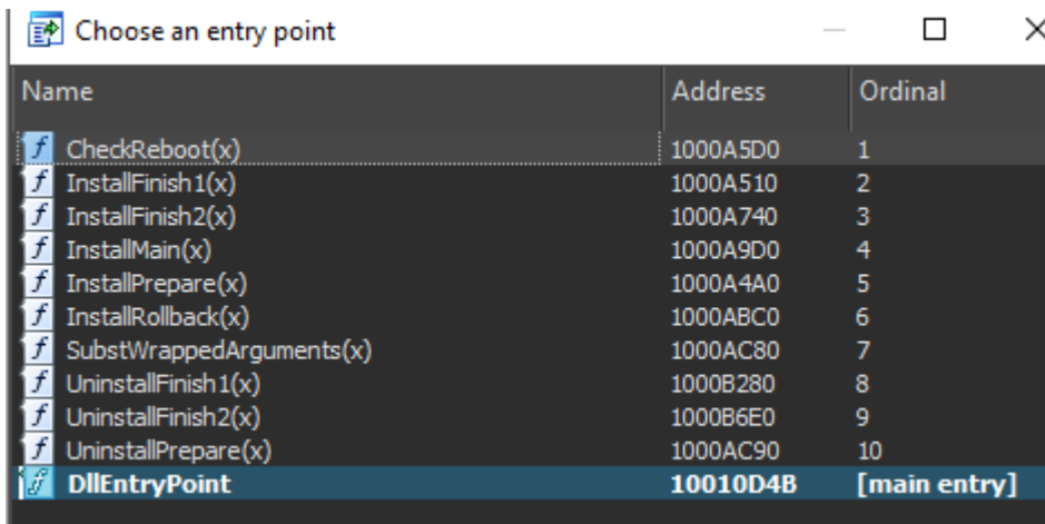
Figure 8: Extracted DLL Entry points
