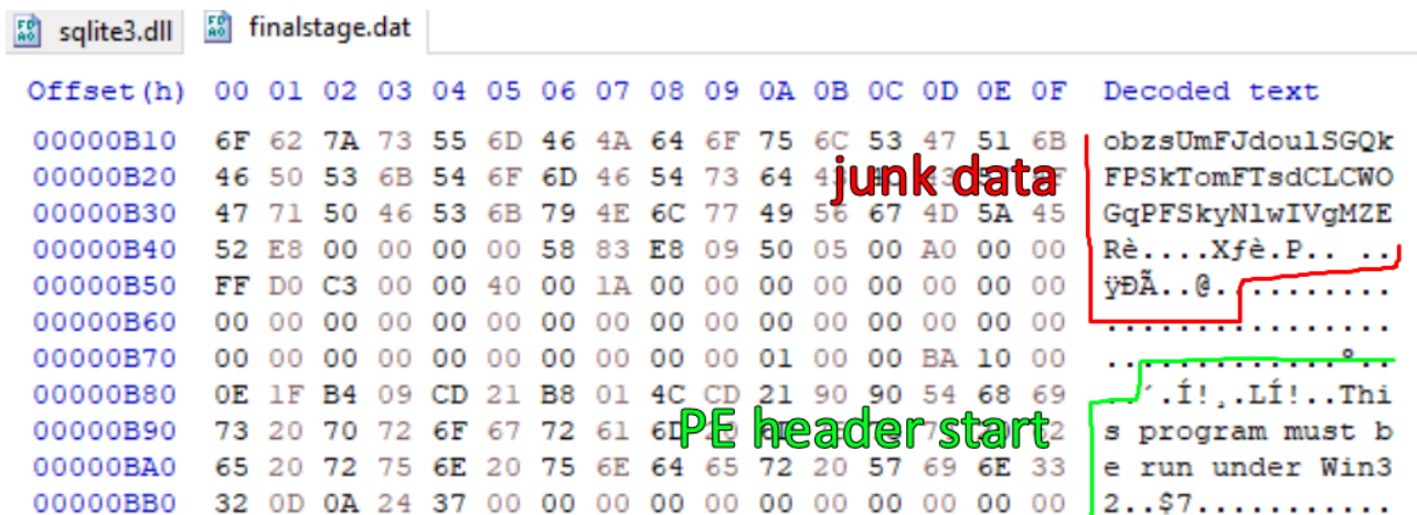
Figure 30: PE Header in Extracted Shellcode File
