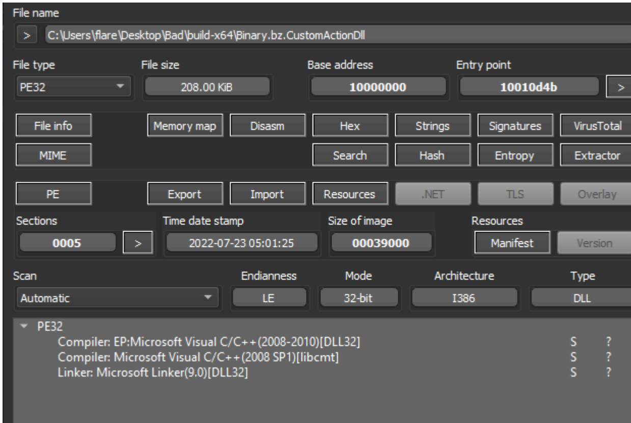
Figure 7: Extracted DLL File in DIE
