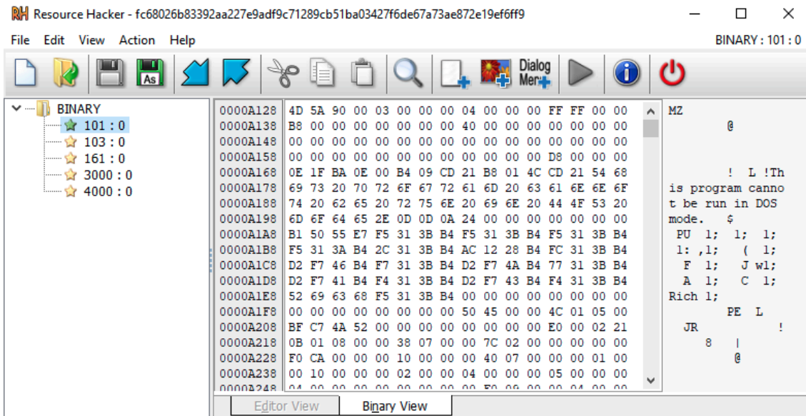
Figure 4. Snake loader’s resources.
