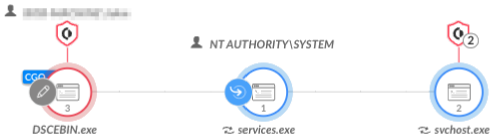
Figure 19. Carbon creates a service that loads the additional components, which is shown in Cortex XDR in detect mode.
