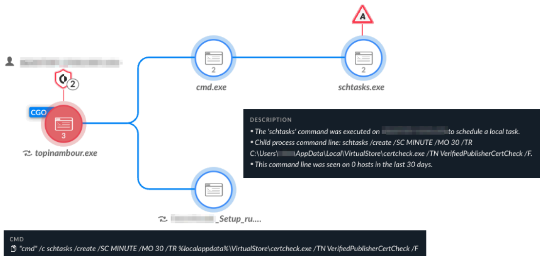
Figure 13. Topinambour execution detection shown in Cortex XDR in detect mode.
