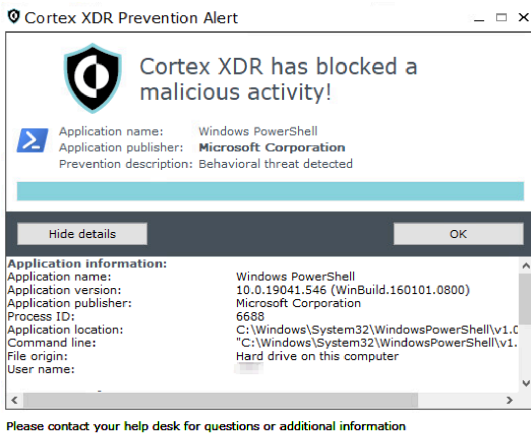
Figure 18a. ComRAT PowerShell dropper execution prevention alert shown in Cortex XDR.
