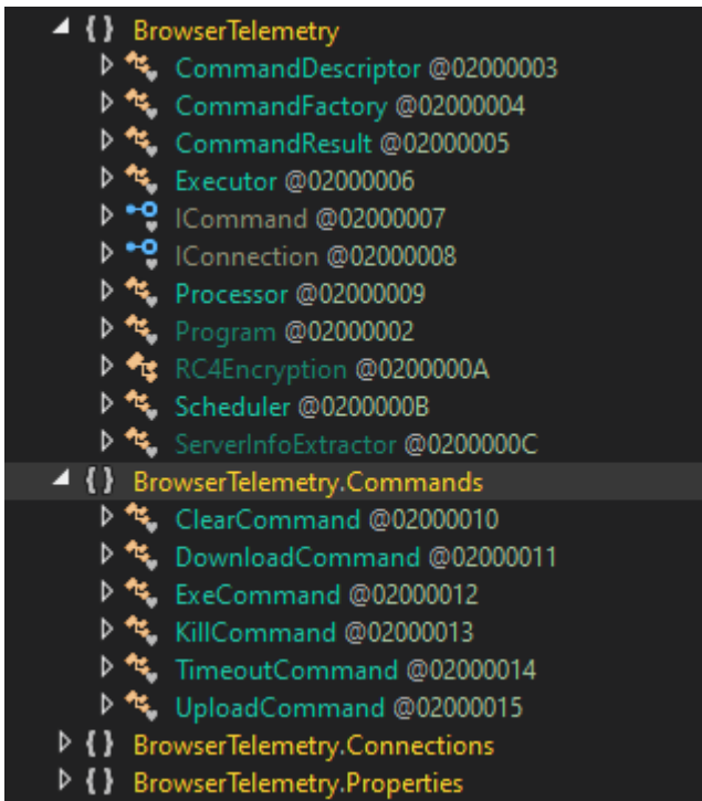
Figure 7. Code snippet of the different classes in QUIETCANARY’s code.
