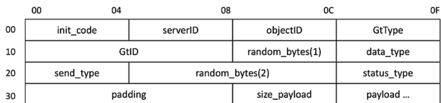
Figure 7. The communication data structures used by Troll Stealer.
