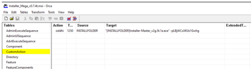
Installer_Mega_v0.7.4t.msi in Orca.exe (click to enlarge)
