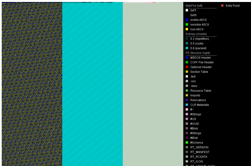
PortexAnalyzer visualization of bloated Installer-Ultimate_v4.3e.9b.exe
