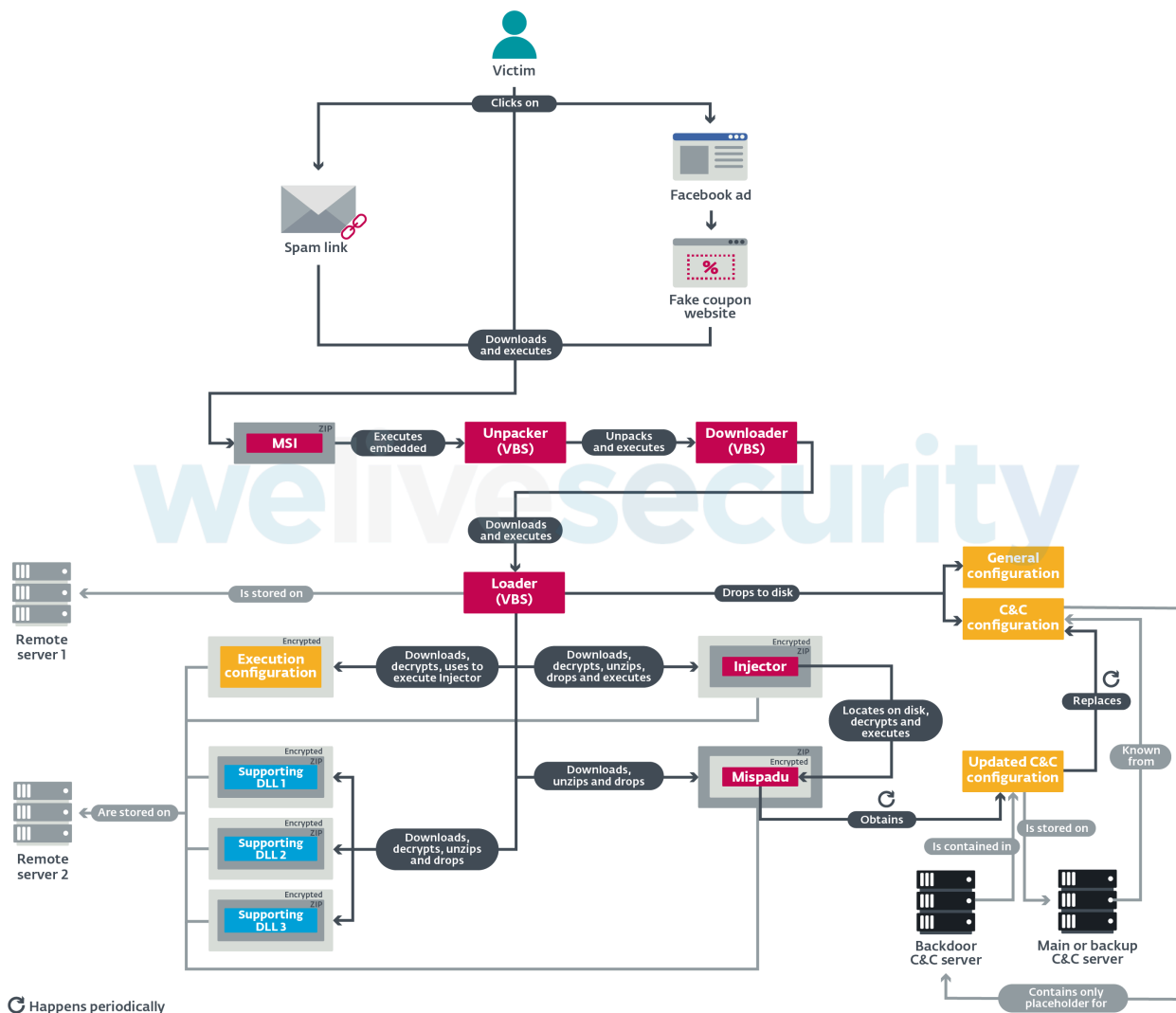
Figure 5. Mispadu’s distribution and execution chain
