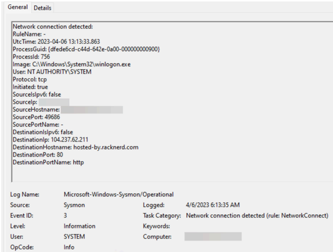
Figure 7: Sysmon event entry indicating winlogon.exe attempting to communicate outbound on port 80
