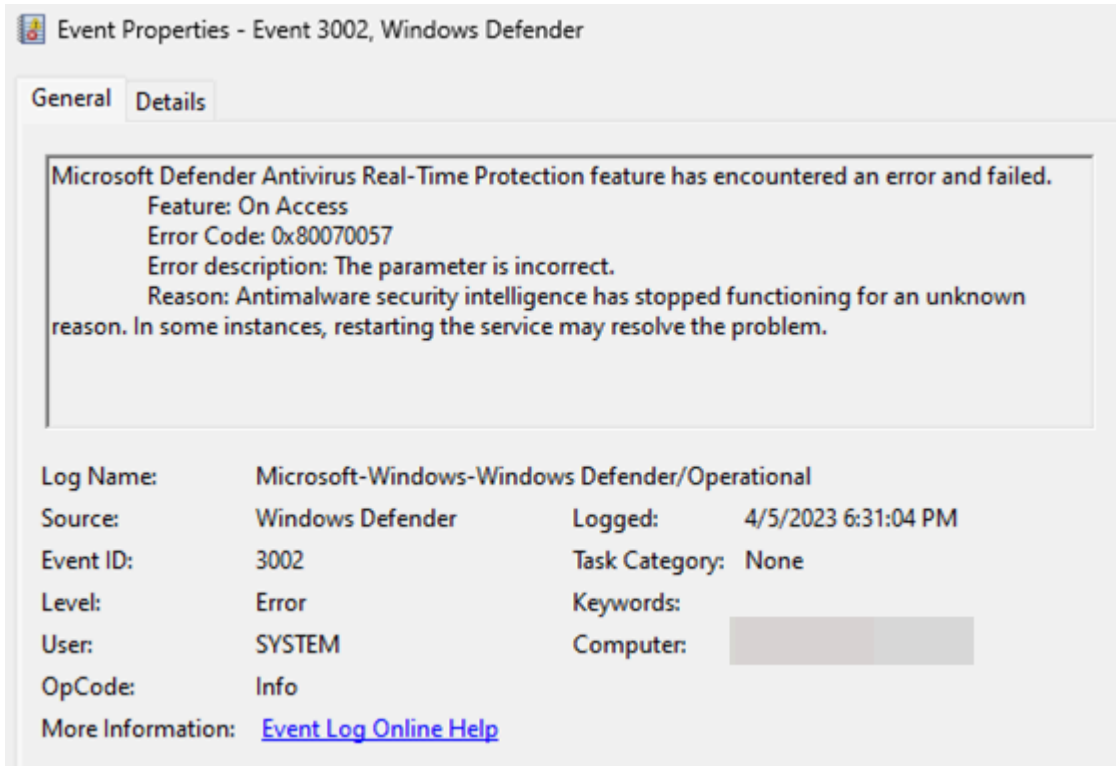
Figure 5: Event Log indicating Microsoft Defender Antivirus real-time protection has stopped functioning
