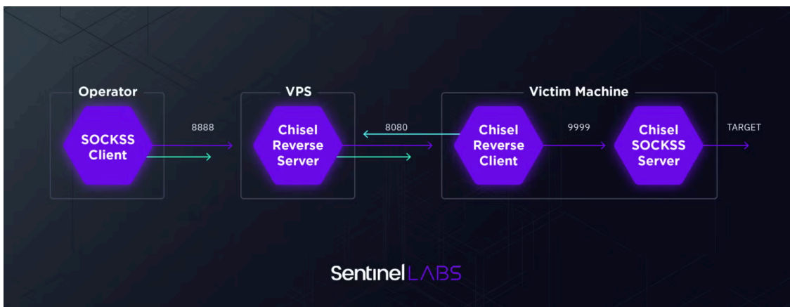
Summary of MuddyWater tunneling using Chisel
