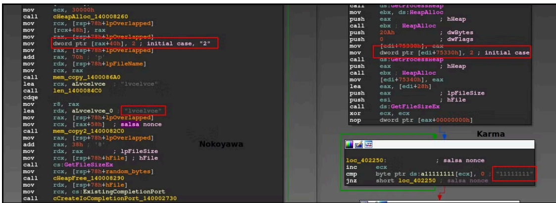
Initial case, encryption thread
