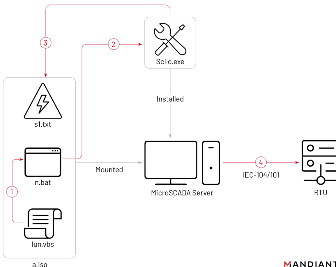
Figure 1: Execution chain of disruptive OT event
