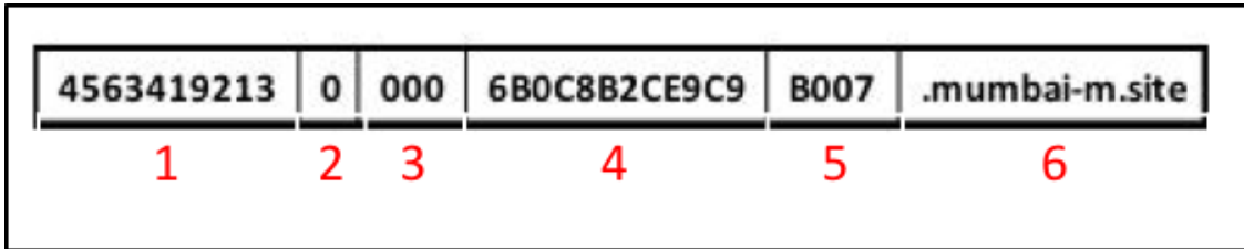
Figure 7: Breakdown of subdomain created by BONDUPDATER
