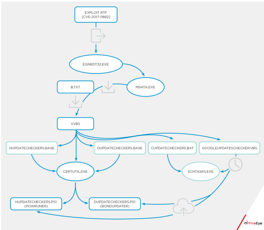
Figure 3: CVE-2017-11882 and POWRUNER attack sequence
