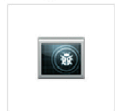
crashreporter.exe
