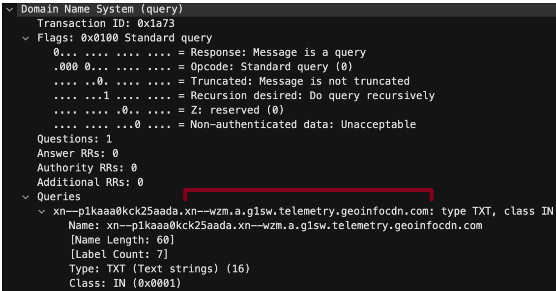
Figure 9. Sample DNS query.
