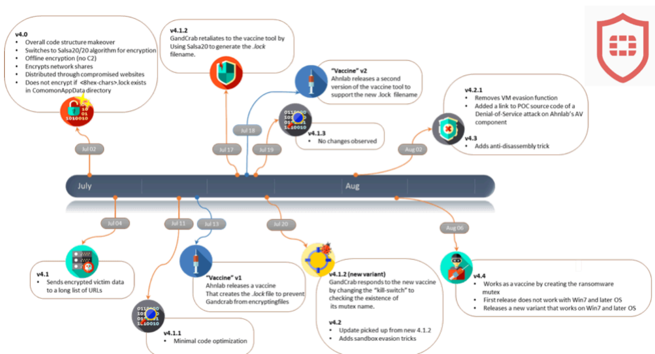
Figure 5: GandCrab v4.0-v4.4 timeline
