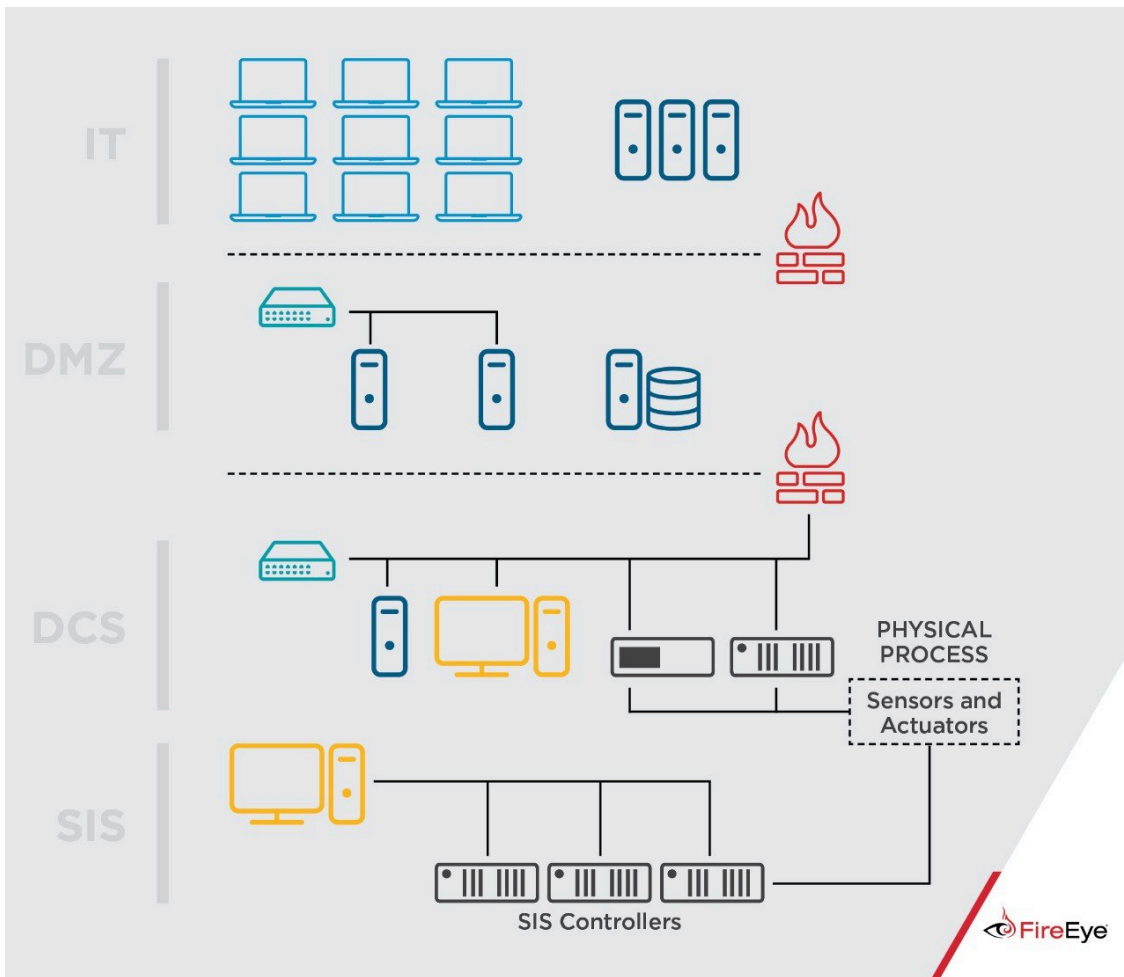
Figure 1: ICS Reference Architecture
