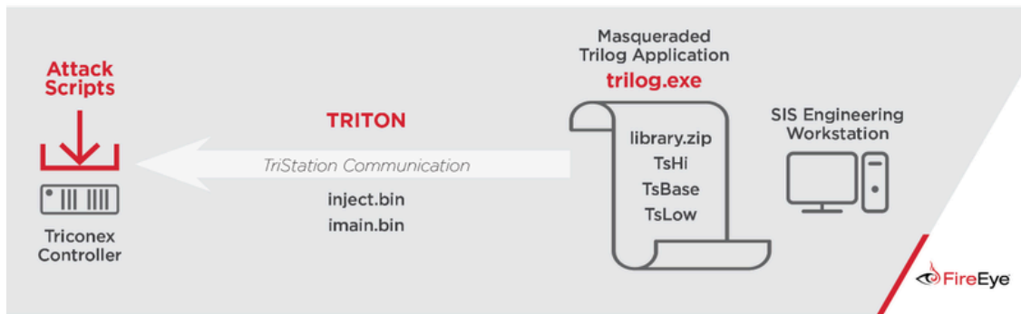
Figure 4: TRITON Architecture and Attack Scenario
