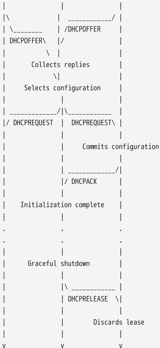
Figure 3: Timeline diagram of messages exchanged between DHCP client and servers when allocating a new network address
