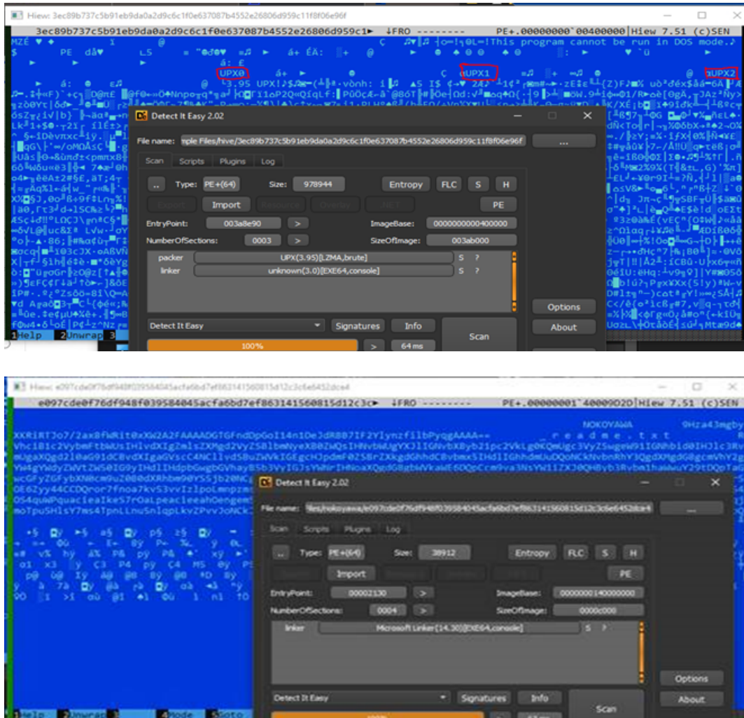
Figure 1. A Hive variant packed using UPX compared to the Nokoyawa sample we analyzed
