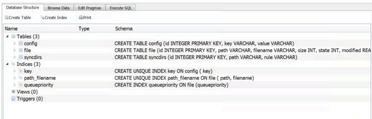
Figure 9: Structure of the local SQLite database
