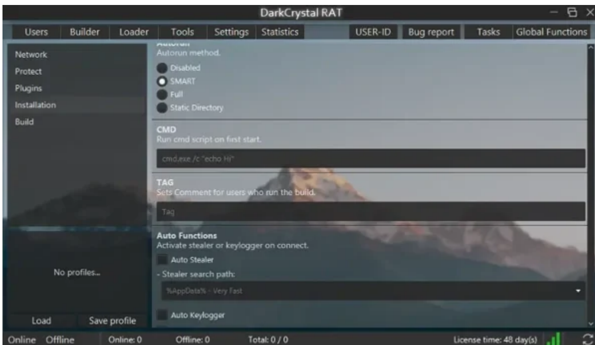
Figure 8 – DarkCrystal RAT
