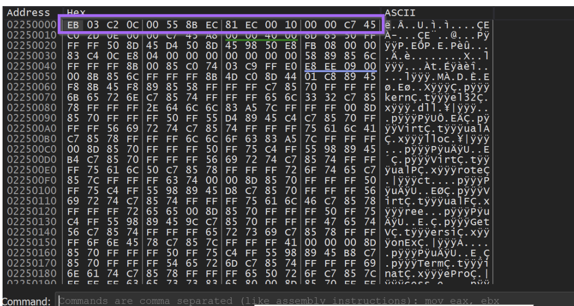
Identifying a Memory Buffer containing Shellcode
