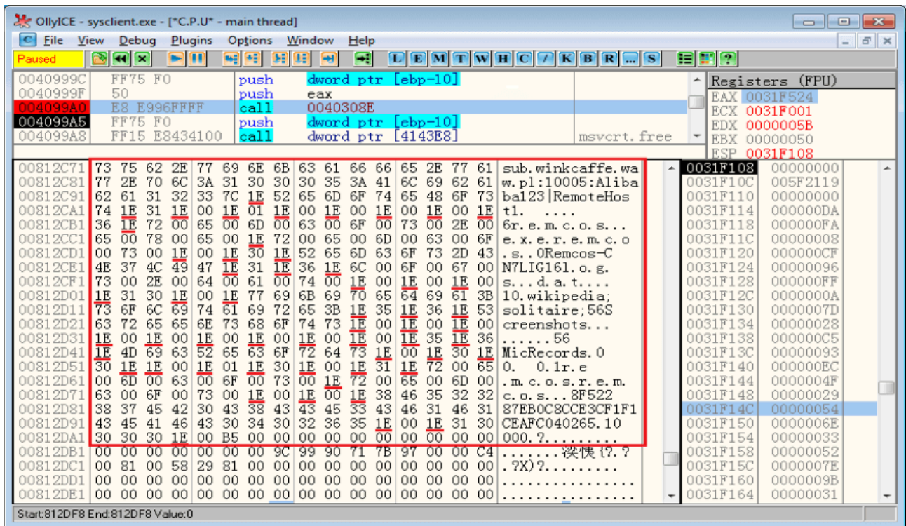
Figure 7. Decrypted resource “SETTINGS”
