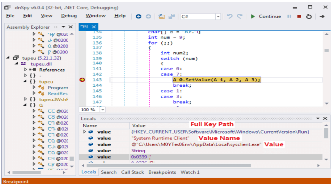
Figure 6. Addition into Auto-Start group of system registry
