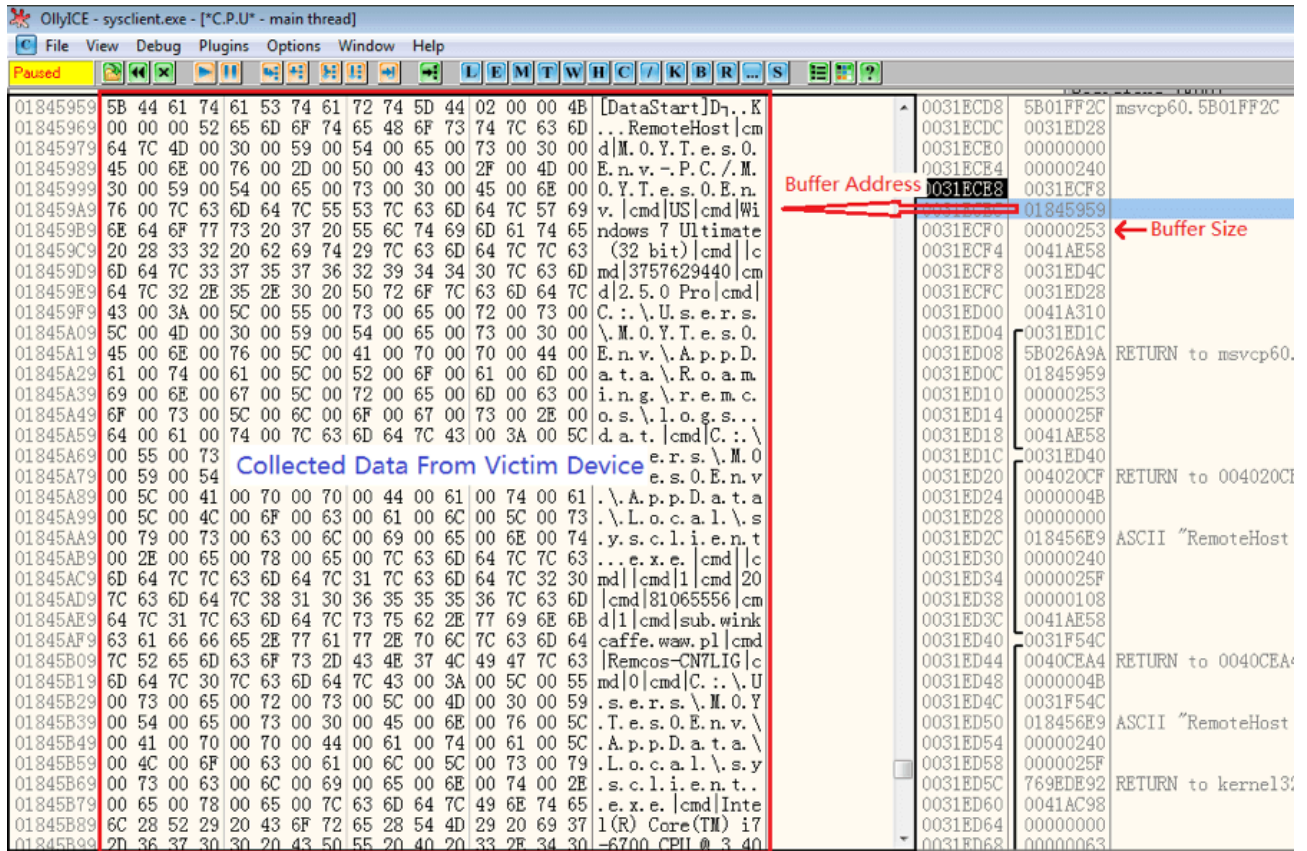
Figure 9. All collected data from victim’s device
