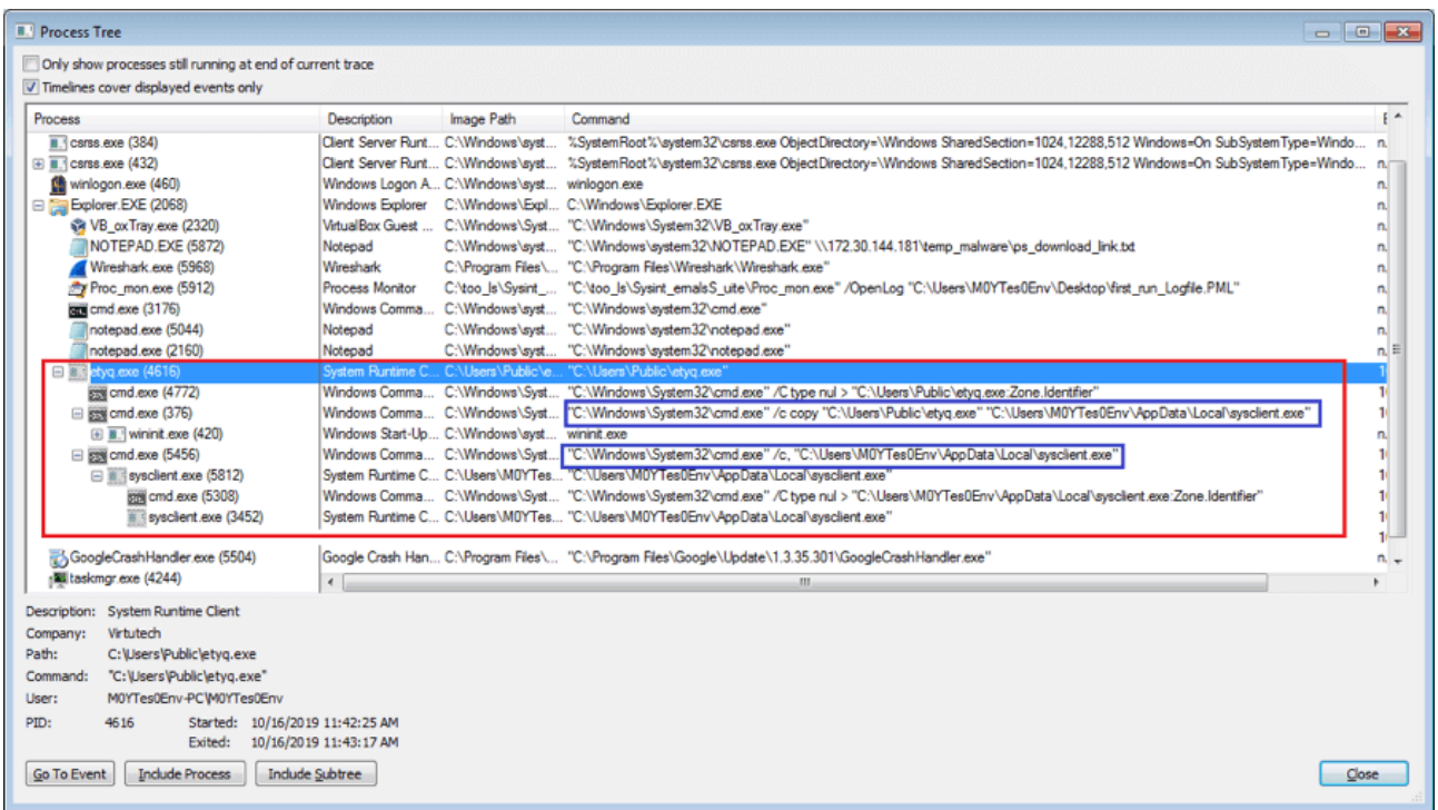
Figure 5. Process tree when first running the dropped Remcos
