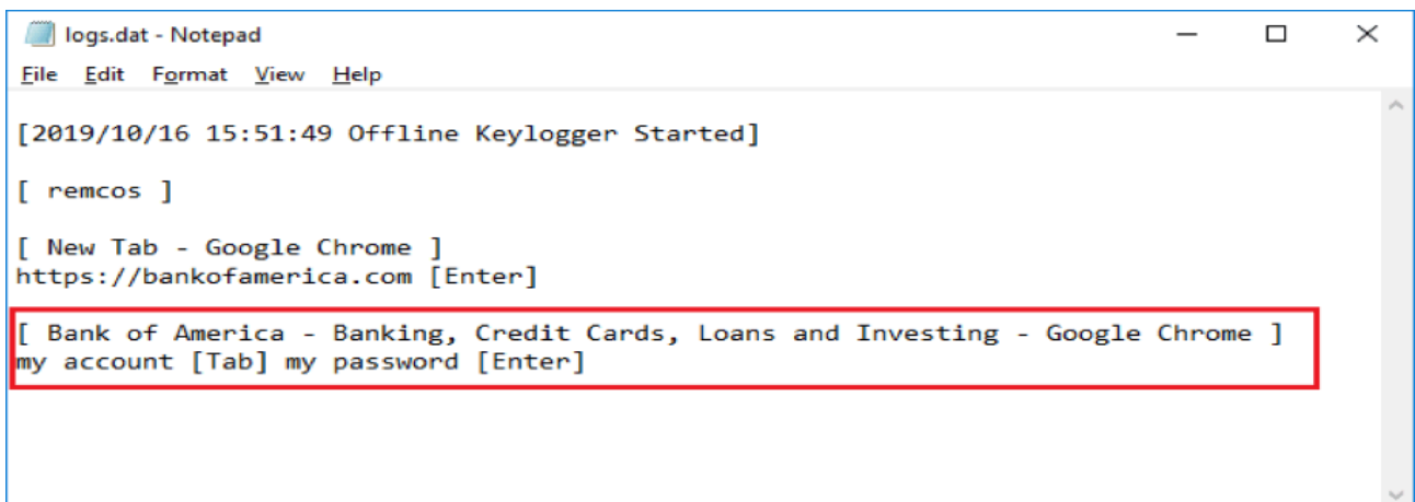
Figure 8. Example Keylogger logs.dat file content
