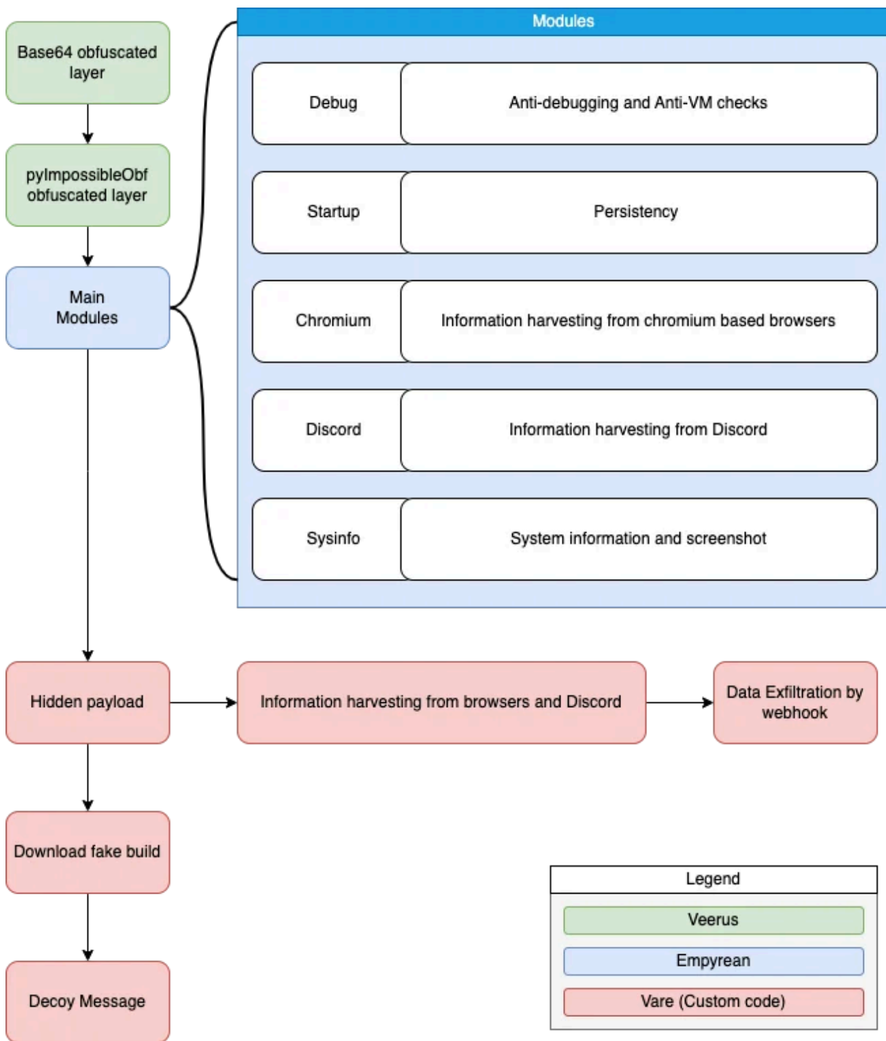
Figure 4: Vare logic flow
