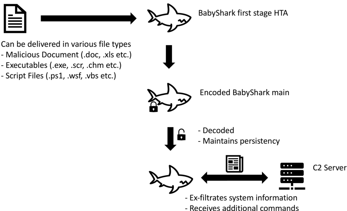
Figure 1 BabyShark execution flow
