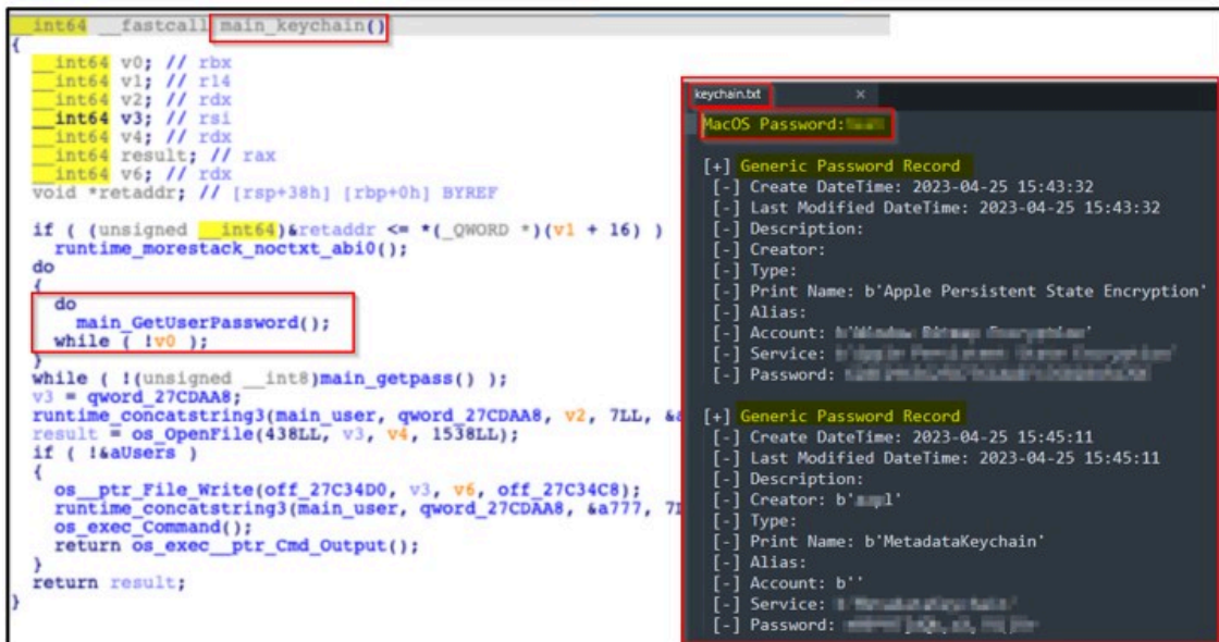
Figure 5 – Keychain password extraction
