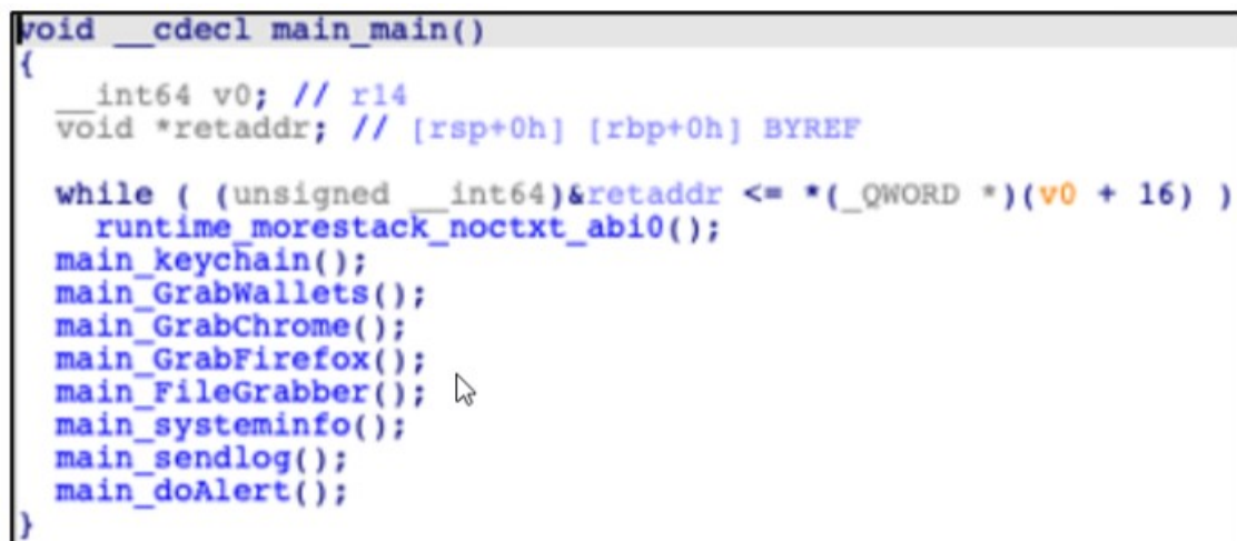
Figure 3 – Stealer’s main function
