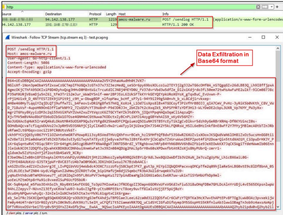
Figure 11 – Exfiltrated data
