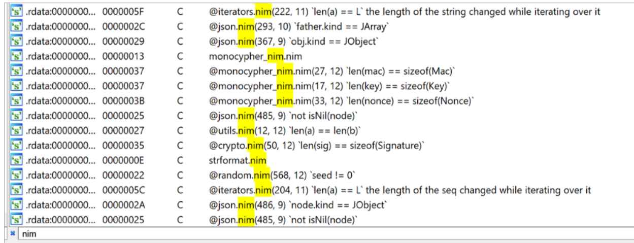
Figure 3: Example of Nim related strings
