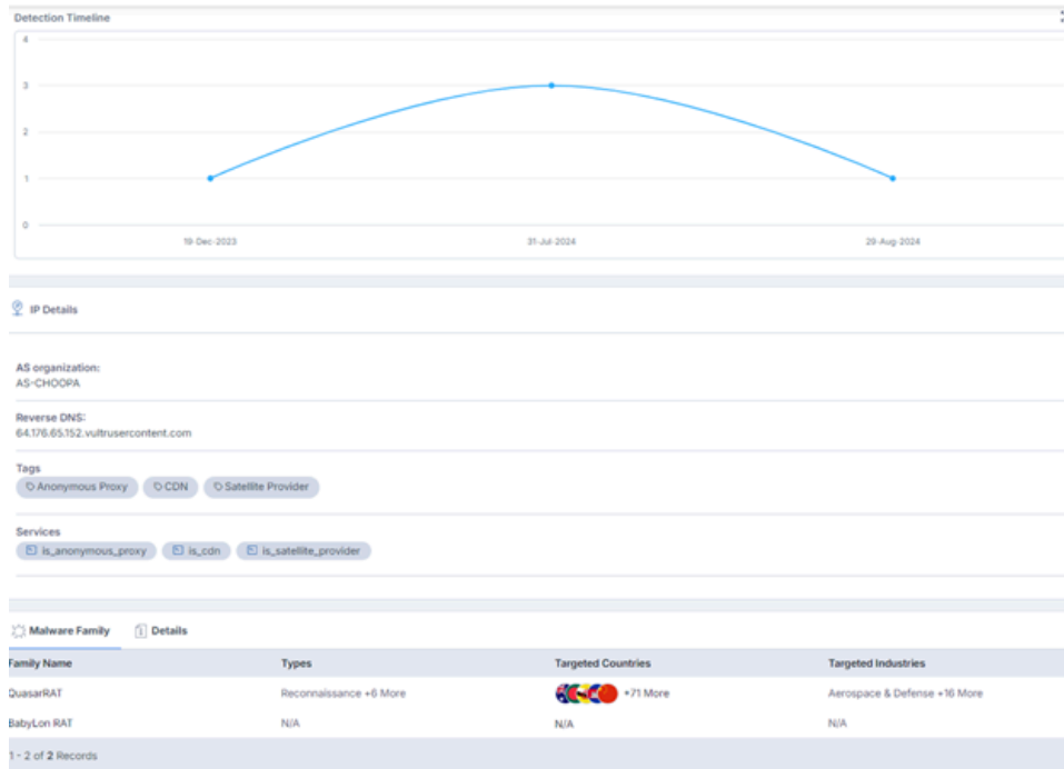
Figure 11 –IP Address 64.176.65.[.]152 Details in Cyble Vision
